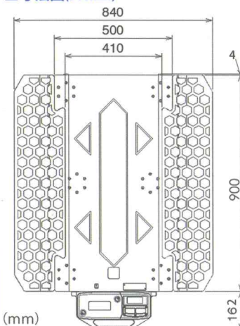
■寸法図(900mm)
